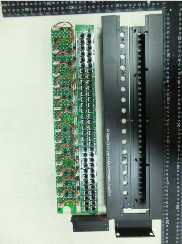
04 Inside Port of EUT
