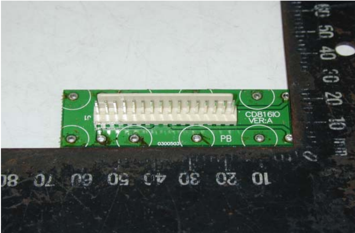
Component Side of Main Board 4
