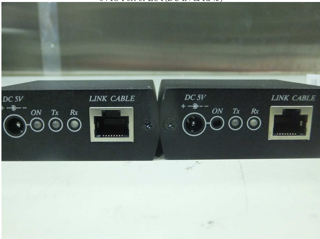
04 IO Port of EUT(DC IN & RJ45)
