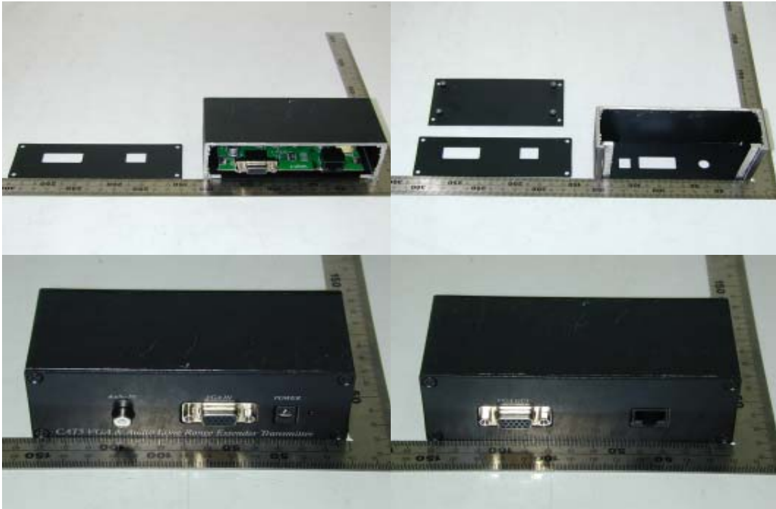
Full View of EUT(Model : VA01XT)
