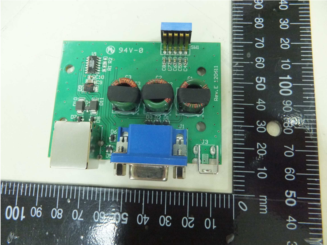
05 Front view of PCB-EUT 1
