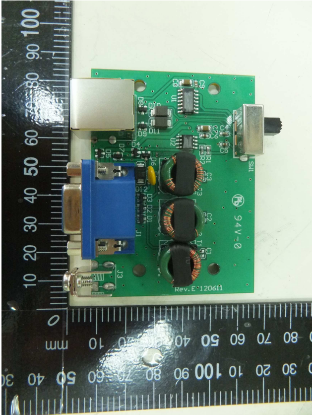
11 Front view of PCB-EUT 2
