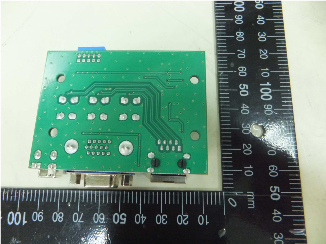
06 Rear view of PCB-EUT 1
