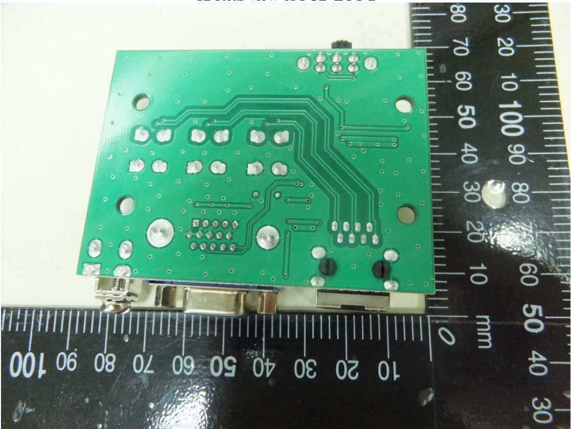
12 Rear view of PCB-EUT 2
