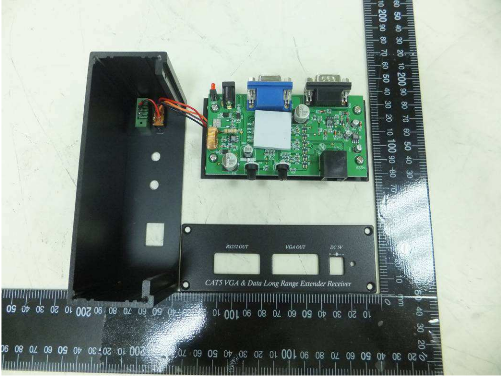
08 EUT2-INSIDE
