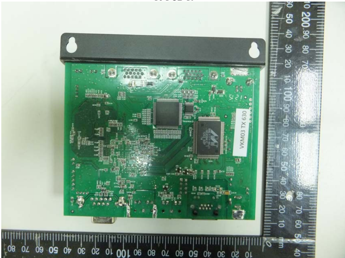
10 PCB-R
