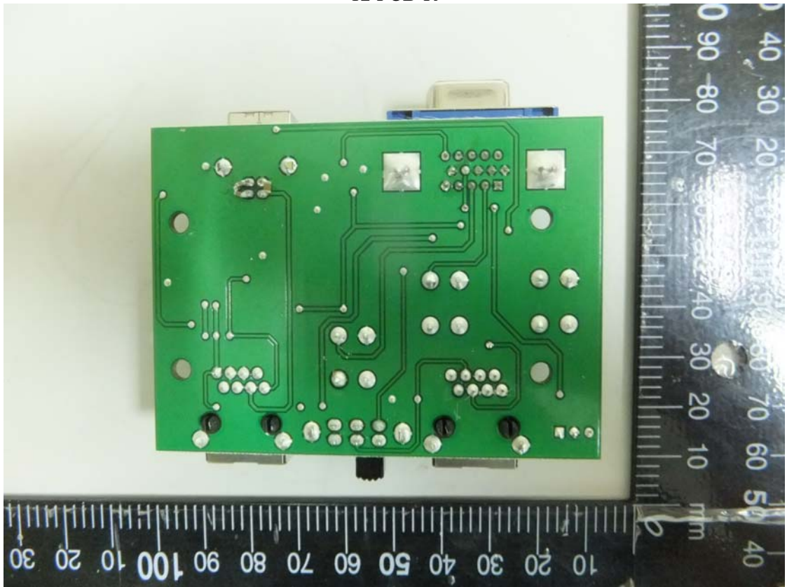
12 PCB-R
