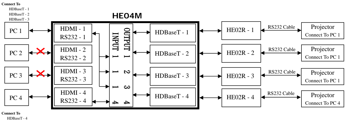
RS-232 SETTING : MATRIX MODE
